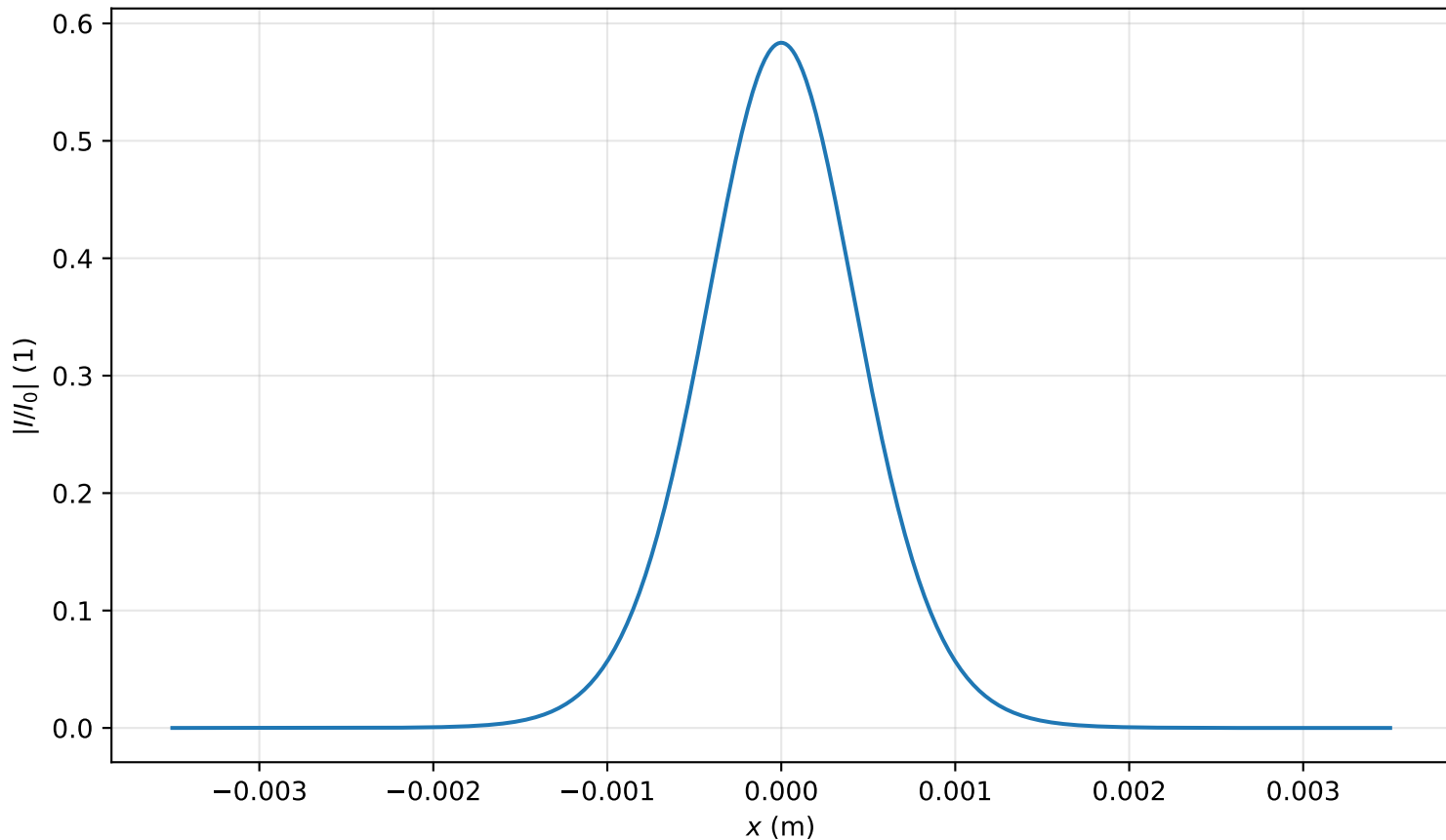
Intensity profile I(x, y = 0, z = 2.548m)/I_0 , P_{in}=0.4P_{cr} , artificial time
